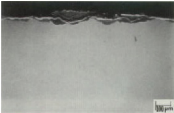
HR-160® alloy
