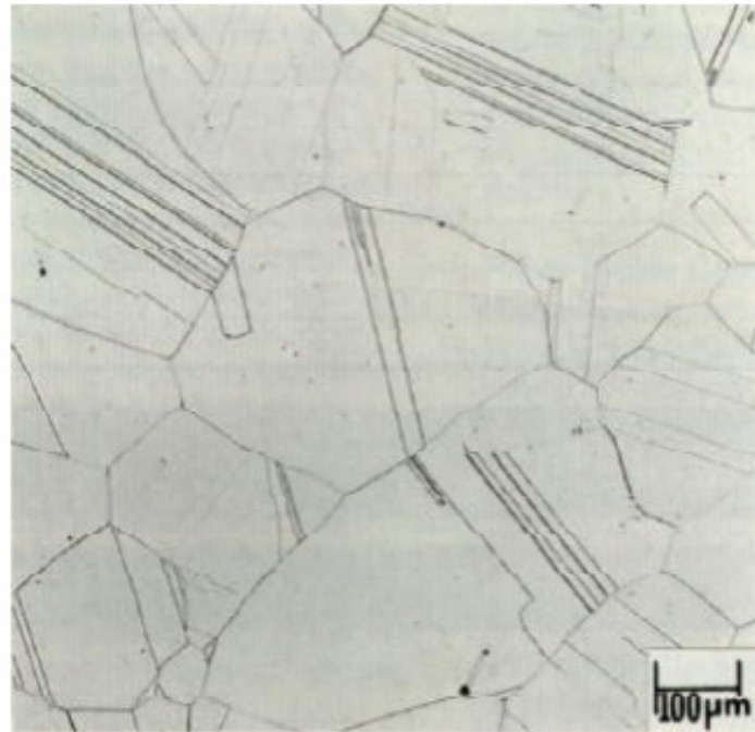
Annealed Microstructure
